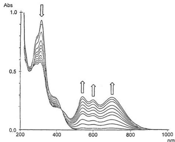
Figure 2. Continuous changes in the UV–vis spectra of 1 upon constant-current electrochemical oxidation (29 \mu\text{A} ) at 2 min intervals in MeCN.
