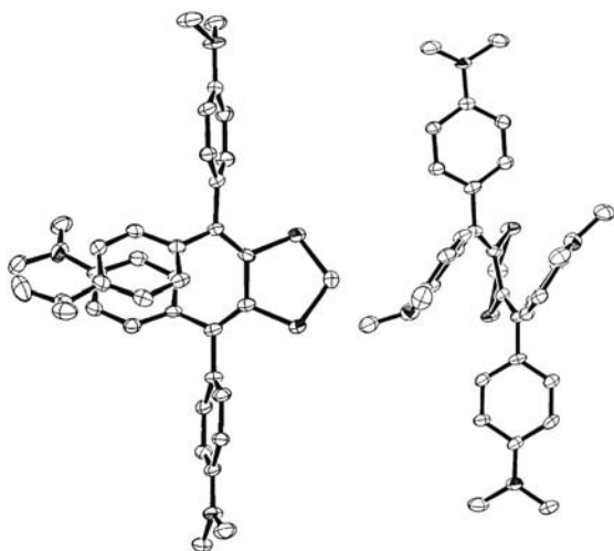
Figure 1. ORTEP drawings of ( P )- 1 (left: top view; right: side view) obtained by X-ray analysis of rac - 1 at 110 K.
